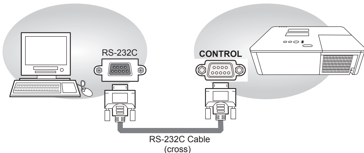
RS-232C port of the computer
